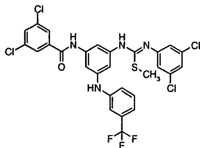
Compound # 9
